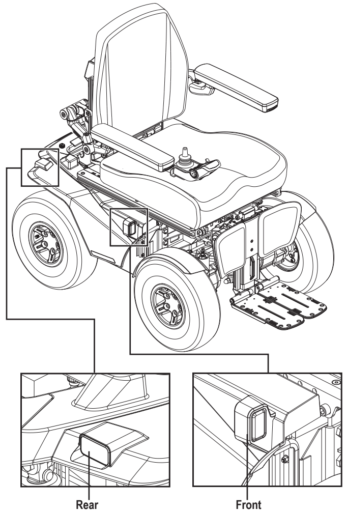
Figure 3. LED Lights
