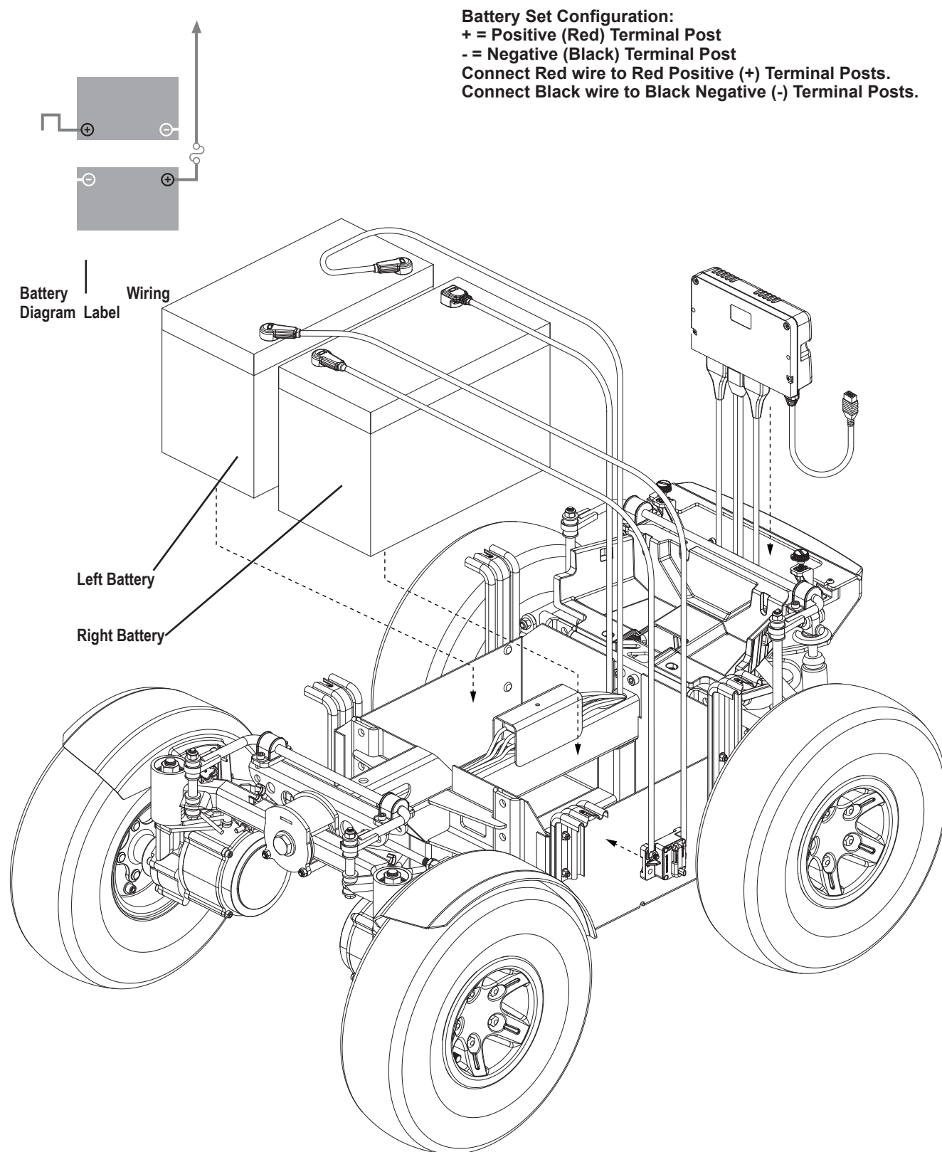
Figure 19. Battery Installation
