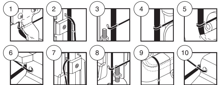
Figure 8. Controller Harness Routing on a Captain's Seat
