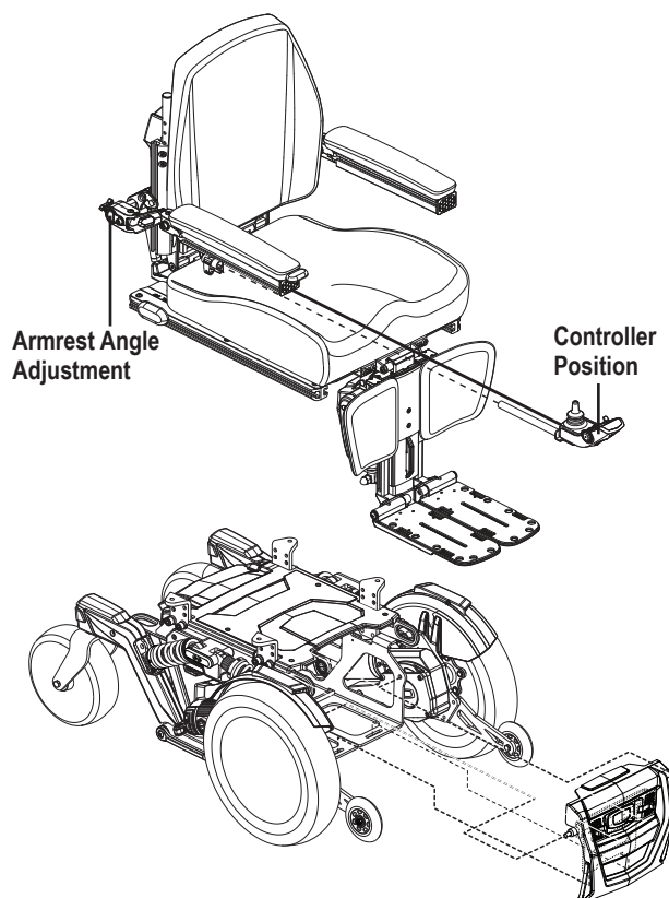
Figure 4. Quantum 4Front Series Assembly View
