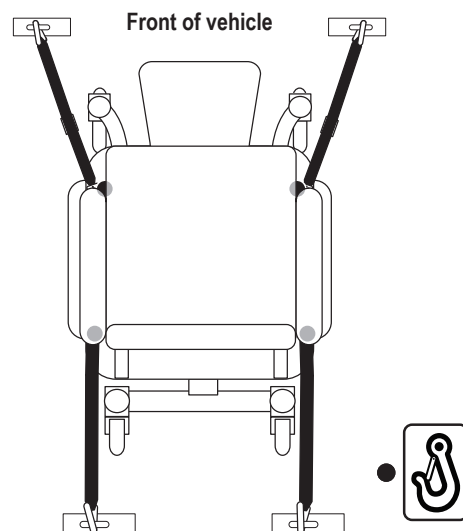
Figure 6. Unoccupied Transit System Securement Points
