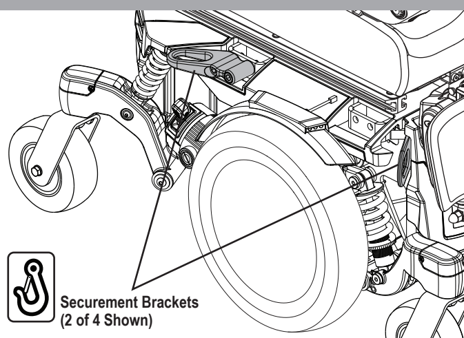
Figure 6. Transit System Securement Brackets
