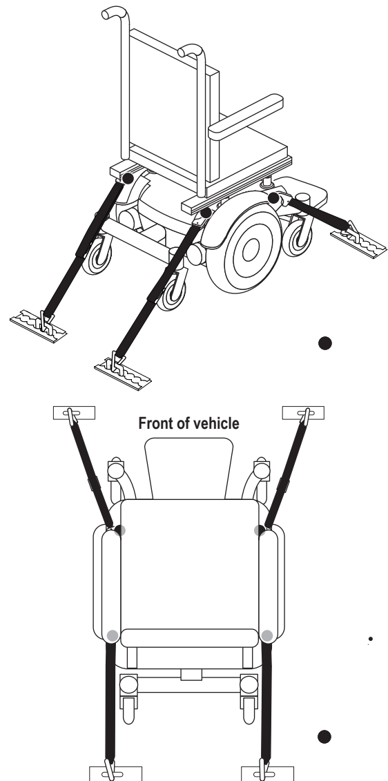
Figure 7. Unoccupied Transit System Securement Points
