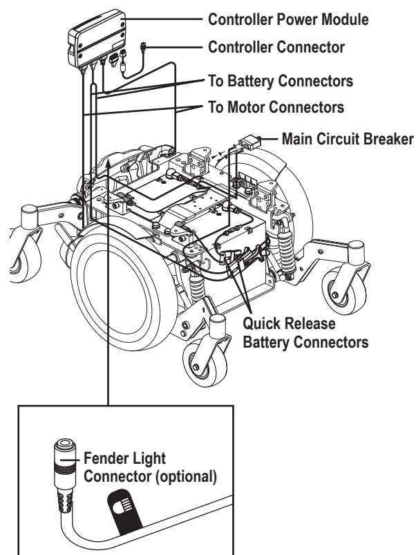
Figure 1. Electrical Components
