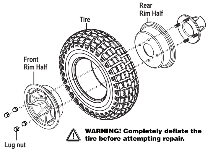
Figure 18. Drive Wheel Disassembled
