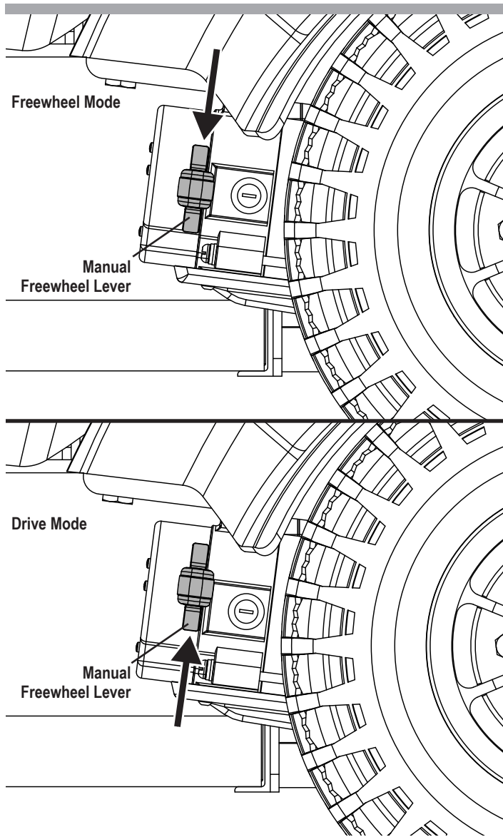
Figure 2. Manual Freewheel Lever Operation
