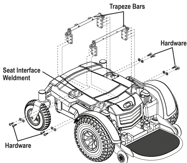
Figure 9. Seat Height/Angle Adjustment
