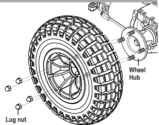
Figure 17. Drive Wheel
