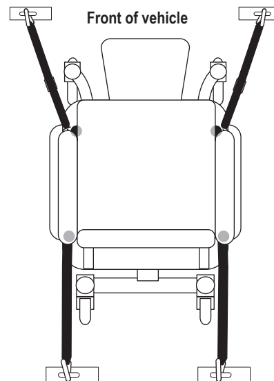
Figure 8. Unoccupied Transit System Securement Points
