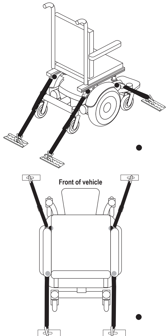
Figure 6. Unoccupied Transit System Securement Points
