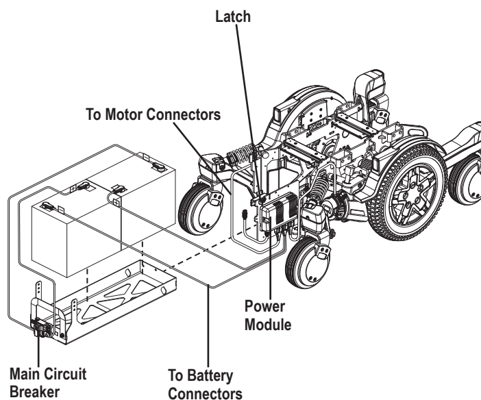
Figure 1. Electrical Components
