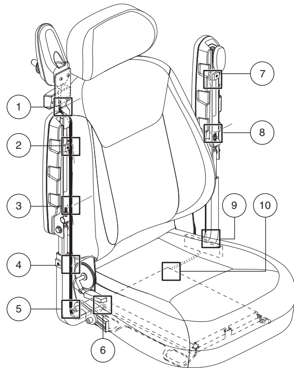
Figure 5. Controller Harness Routing on a TRU-Balance® 4
