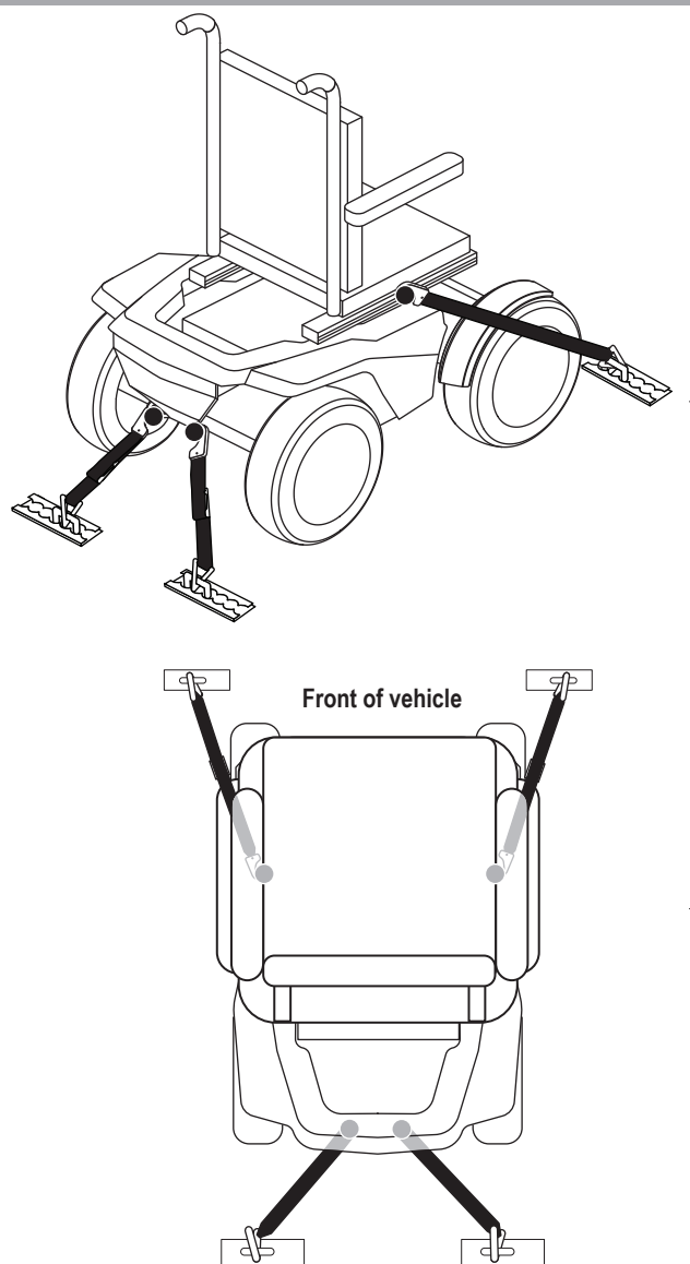
Figure 9 Unoccupied Transit System Securement Points
