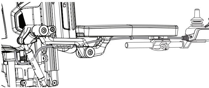
Figure 5. Controller Harness Routing on a TRU-Balance® 4
