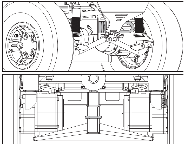
Figure 11. Unoccupied Transit System Securement Points
