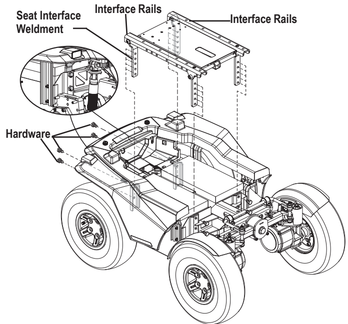
Figure 12. Seat Height/Angle Adjustment
