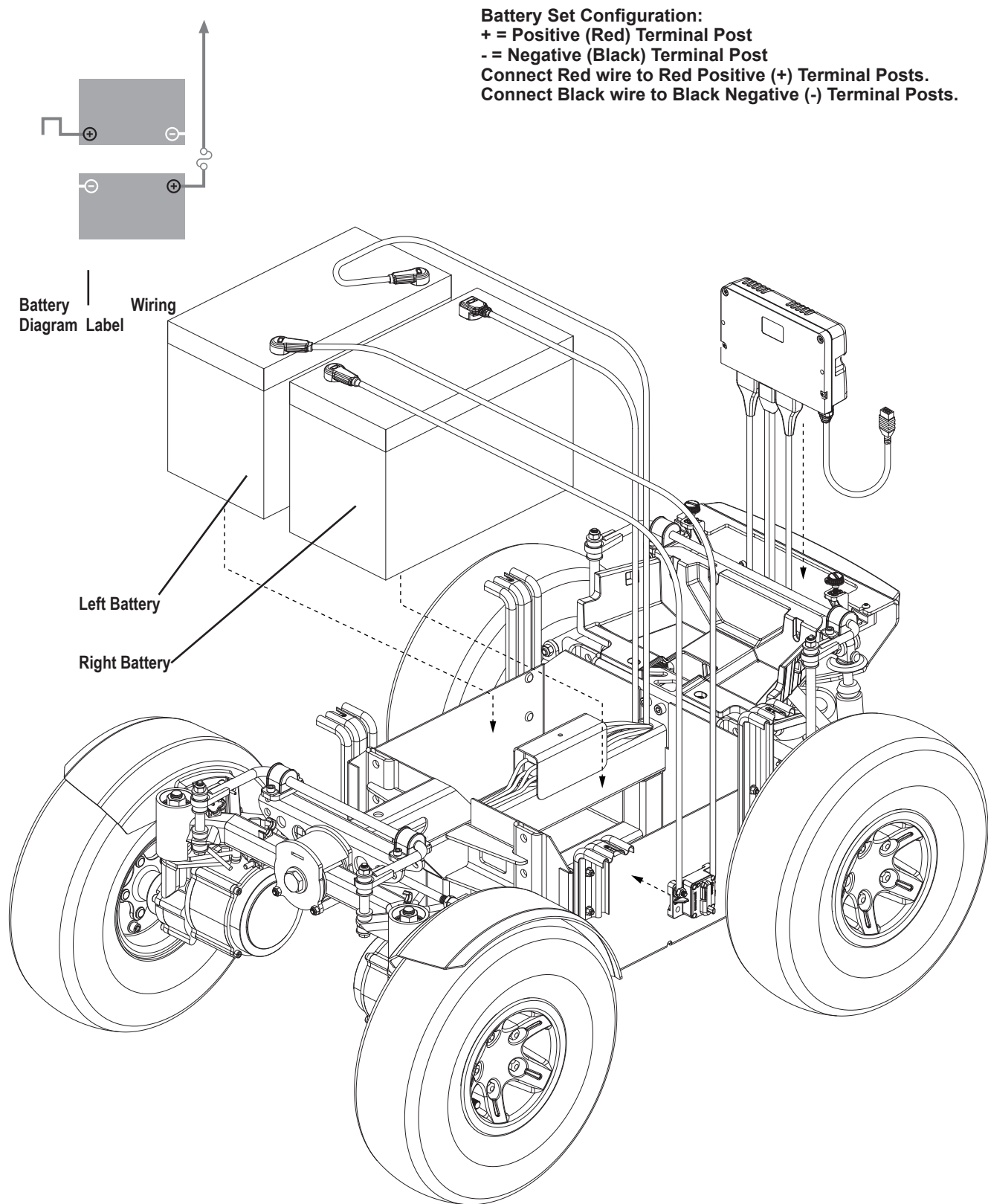
Figure 21. Battery Installation
