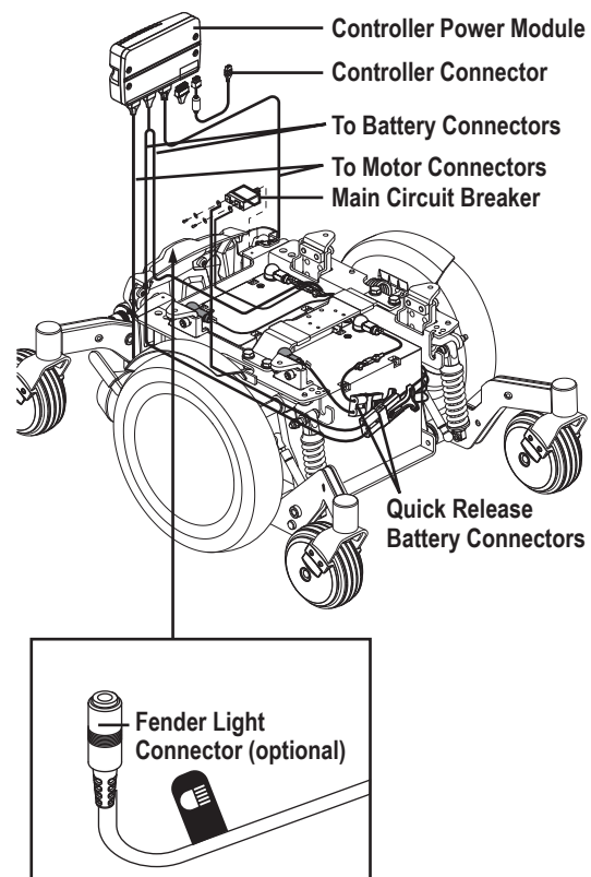
Figure 1. Electrical Components
