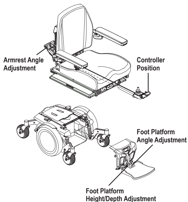
Figure 5. Assembly View
